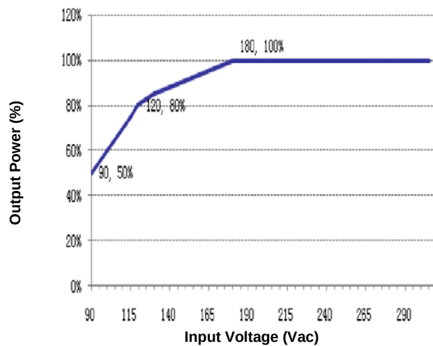
Figure 6: Output Power vs. Input Voltage (Ta = 50°C)
